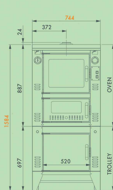
Medium CIBUS oven for interior use (FM)
