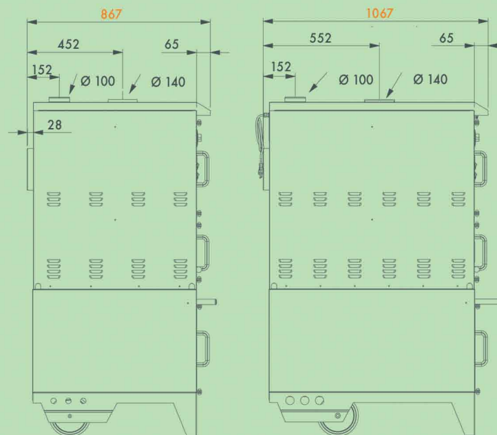
Medium CIBUS oven for interior use (FM)
