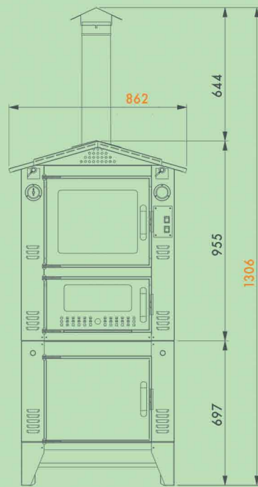
CIBUS oven for exterior use (FM FG)
